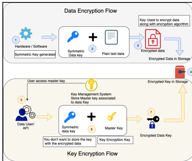
Envelope encryption
