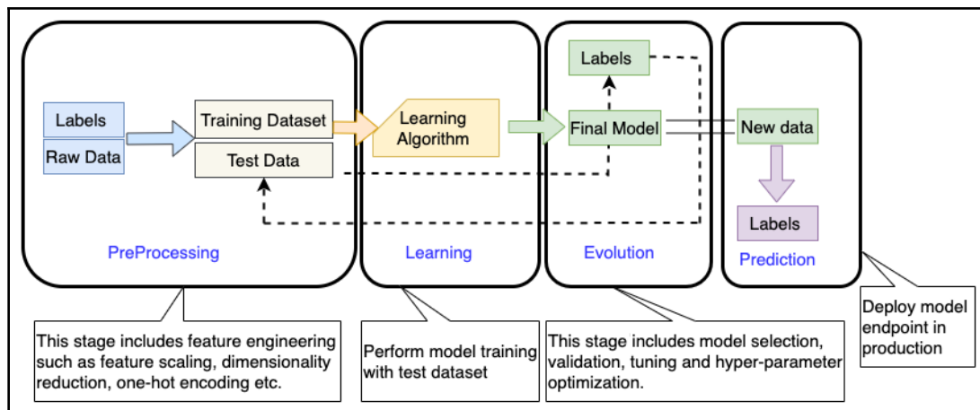
ML workflow
